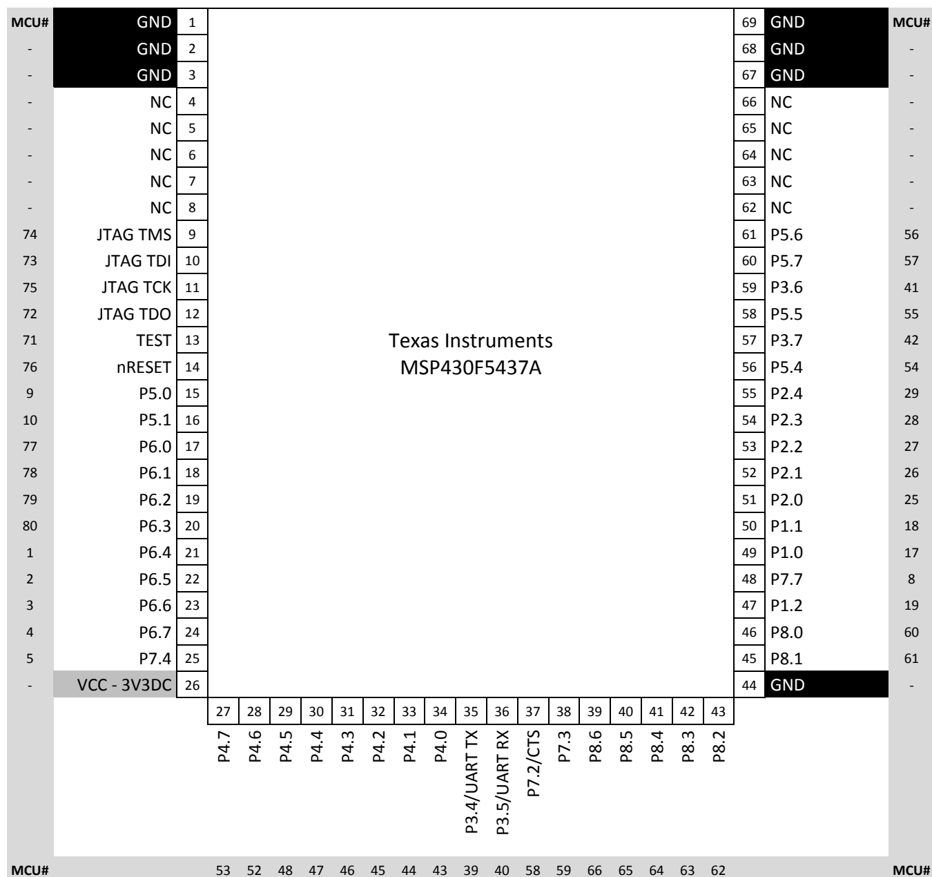
Figure 3 Module Pinout
