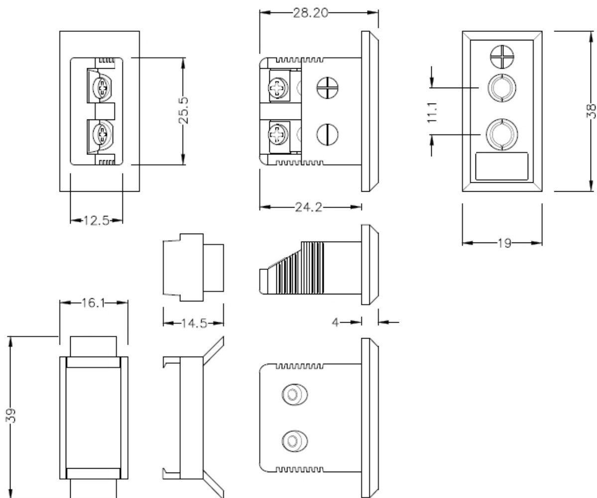
Standard Fascia Socket (with nylon mounting clip) (dimensions in mm)
