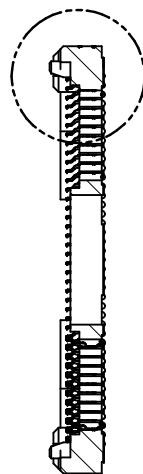
SECTION Z-Z
