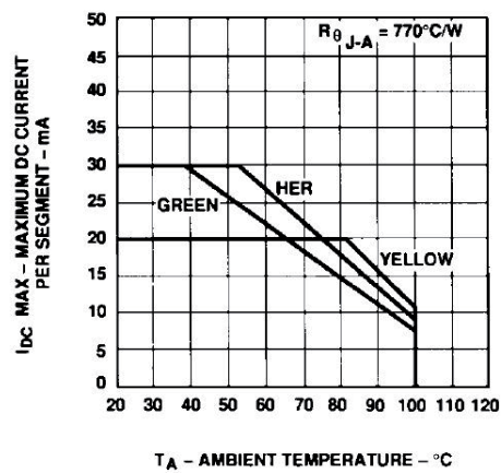
Figure 9. Maximum Allowable DC Current vs. Ambient Temperature.
