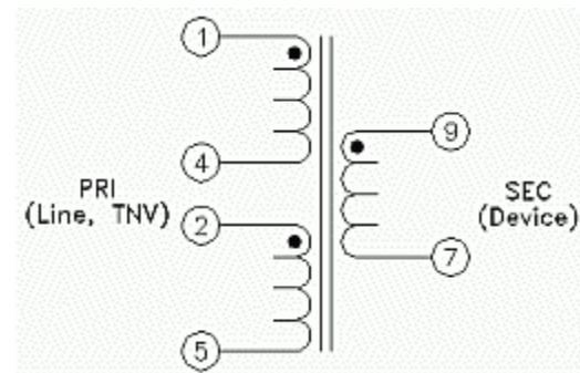
Schematic 2
