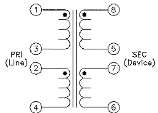
Schematic 4
