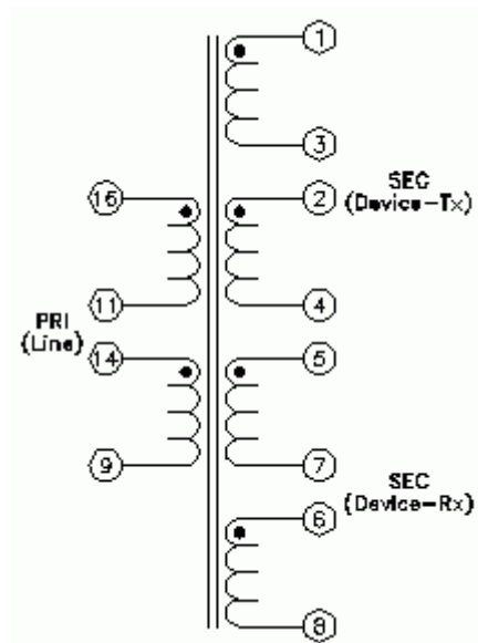
Schematic 1
