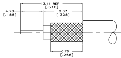
VIEW A RECOMMENDED STRIP LENGTH
