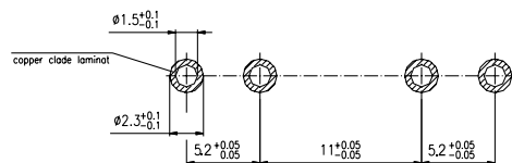
Mounting Dimensions
