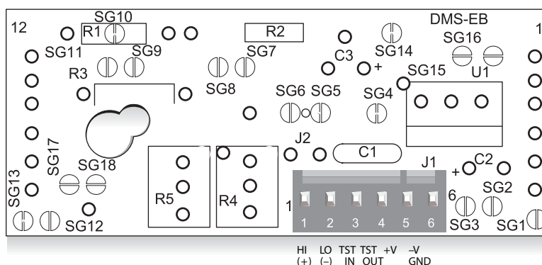
Figure 4. DMS-EB Board
