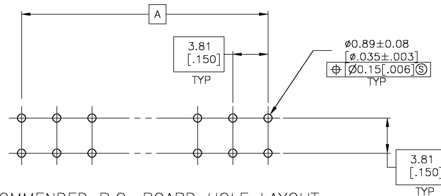
RECOMMENDED P.C. BOARD HOLE LAYOUT
