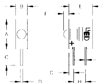
RIGHT ANGLE (WITH STANDOFF) 555M-2XXX
