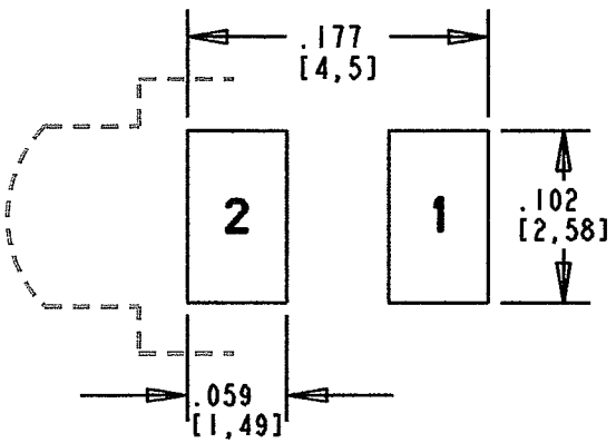
COMPONENT SIDE RECOMMENDED PC BOARD LAND PATTERN (DIM'S ±.004)
