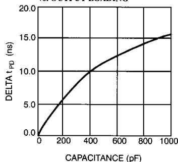
DELTA CLOCK-TO-OUTPUT TIME vs. OUTPUT LOADING
