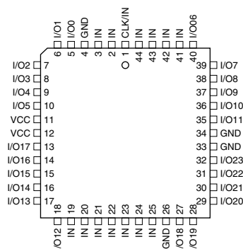
LCC/PLCC
