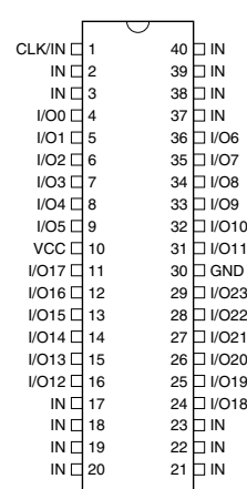
DIP
