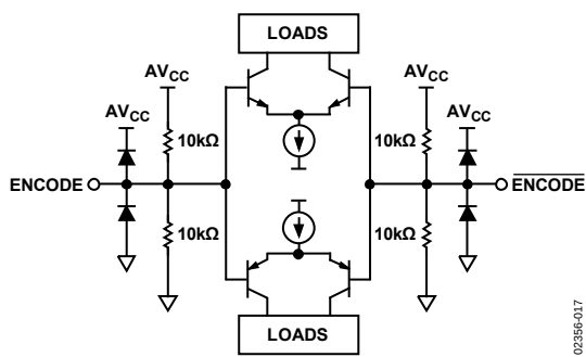
Figure 4. ENCODE Inputs
