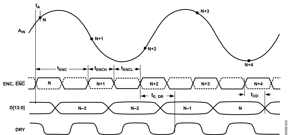
Figure 2. Timing Diagram
