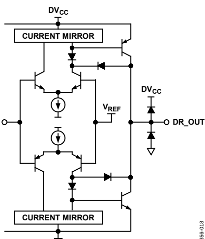
Figure 5. Digital Output Stage
