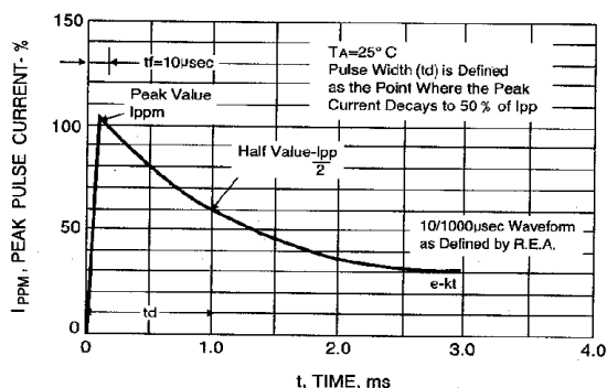
FIGURE 3-PULSE WAVEFORM
