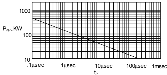
Peak Pulse Power ( P_P ) – versus – Pulse Time ( t_P )
