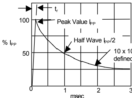
Peak Pulse Current ( \% I_P ) - Versus - Time (t)
