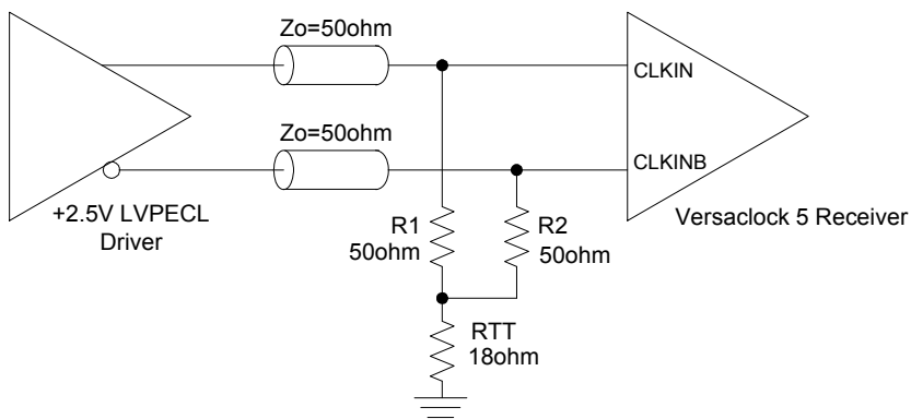
CLKIN, CLKINB Input Driven by a 2.5V LVPECL Driver
