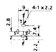
P.C.B. LAYOUT (BOTTOM VIEW)
