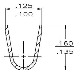
SECTION Y-Y SCALE 10:1
