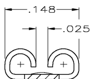
VIEW Z-Z SCALE 10:1
