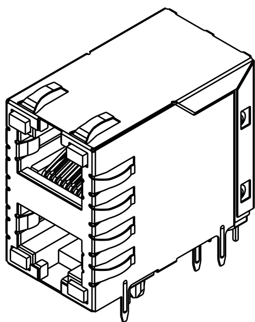
PN 6368011-1,2,3,4,5,6,8 & 1-6368011-0,1,5 SCALE 2:1
