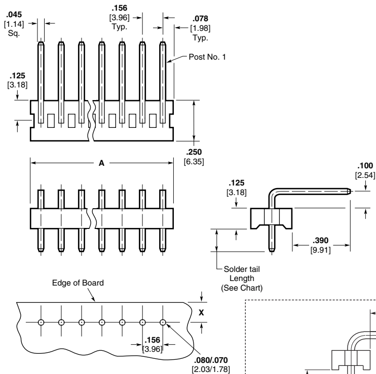
Recommended Mounting Hole Pattern for .062 [1.57] Thk. PC Board
