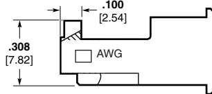
with Polarizing Tabs
