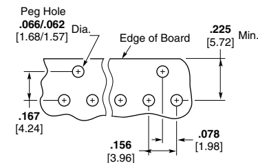
Recommended Mounting Hole Pattern for .062 [1.57] Thk. PC Board
