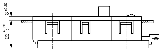
Variants 6424.0X5X.XX Mounting hole: 57^{+0.2}_0 \times 27.6^{+0.2}_0 A: Quick-connect terminal 6.3x0.8 mm: 18.1 mm A: Solder terminal 3.5x0.8 mm: 13.3 mm
