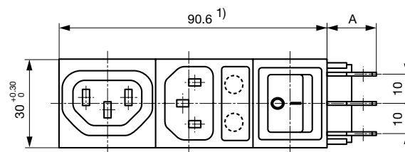
Variants 6432.0X5X.XX Mounting hole: 90.6^{+0.2}_0 \times 27.6^{+0.2}_0 A: Quick-connect terminal 6.3x0.8 mm: 18.1 mm A: Solder terminal 3.5x0.8 mm: 13.3 mm
