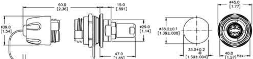
PRO BEAM Sr. D-Hole Bulkhead with Standard Cable Adapter
