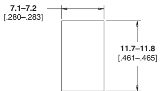
Recommended Panel Cutout Panel Thk. 1.2/1.7 [.047/.067]
