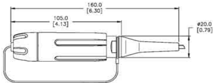
PRO BEAM Jr. Cable Connector, Plug
