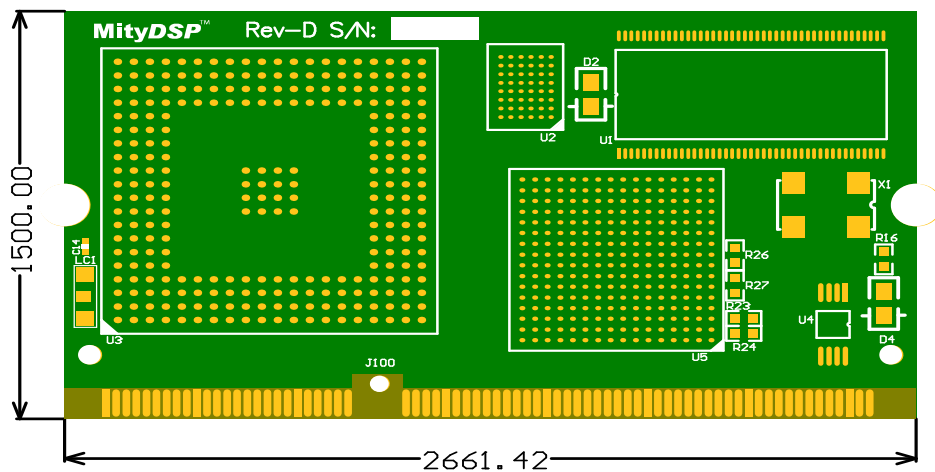
Figure 3 MityDSP Mechanical Outline
