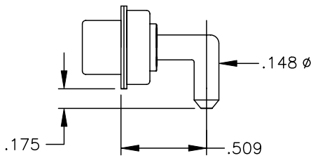
20/40 AMP POWER CONTACTS
