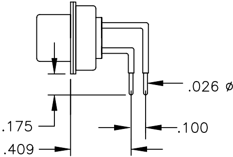
SIGNAL CONTACTS
