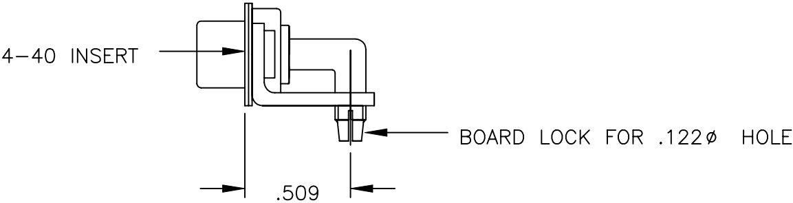
MOUNTING HARDWARE
