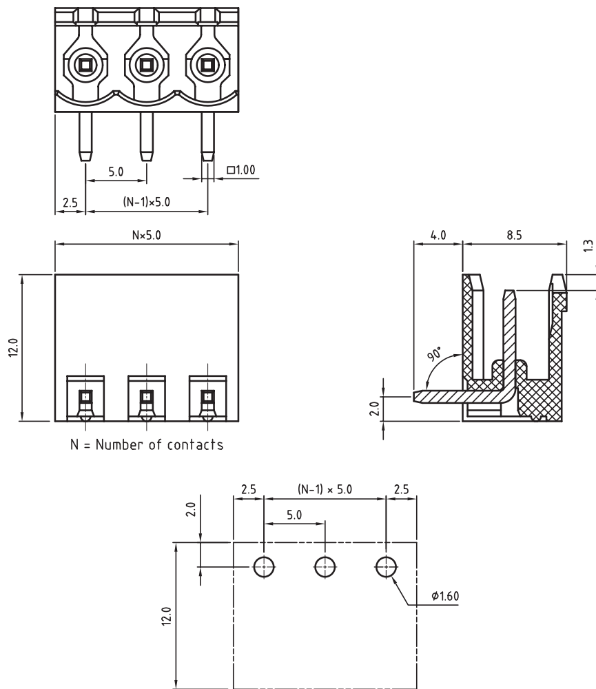
PCB LAYOUT - COMPONENT VIEW
