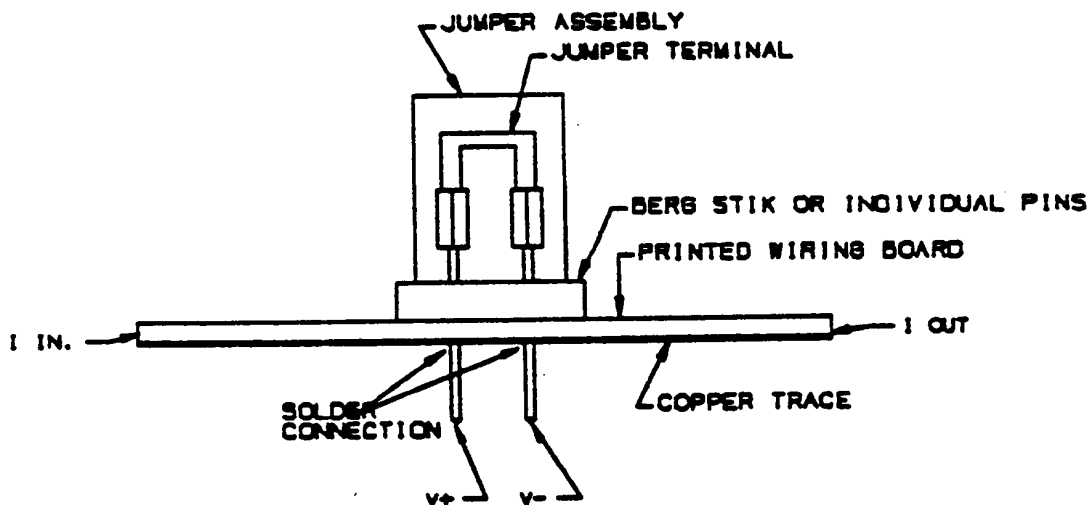
FIGURE 1 - CONTACT RESISTANCE
