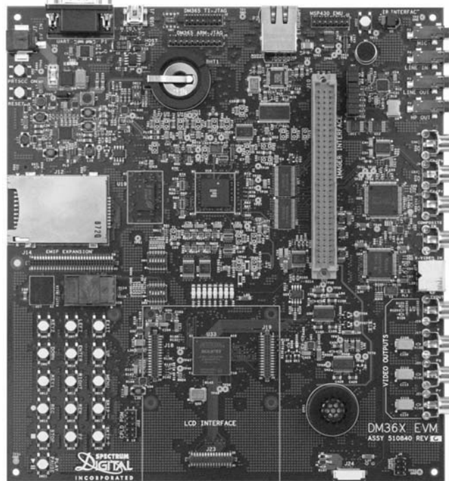
Figure 1-2, DM365 EVM
