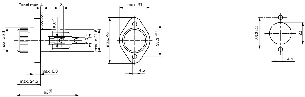
Mounting holes
