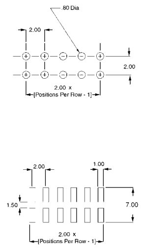
Recommended PCB layouts
