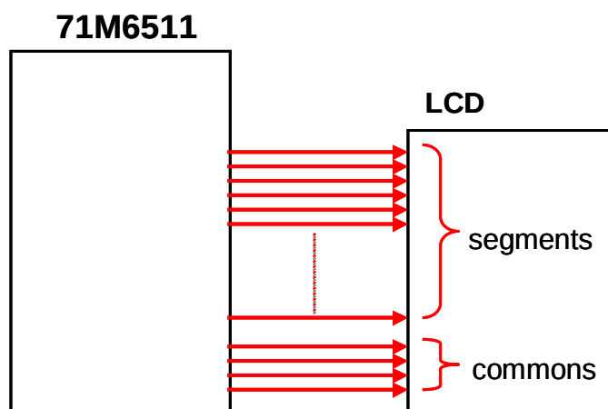
Figure 31: Connecting LCDs
