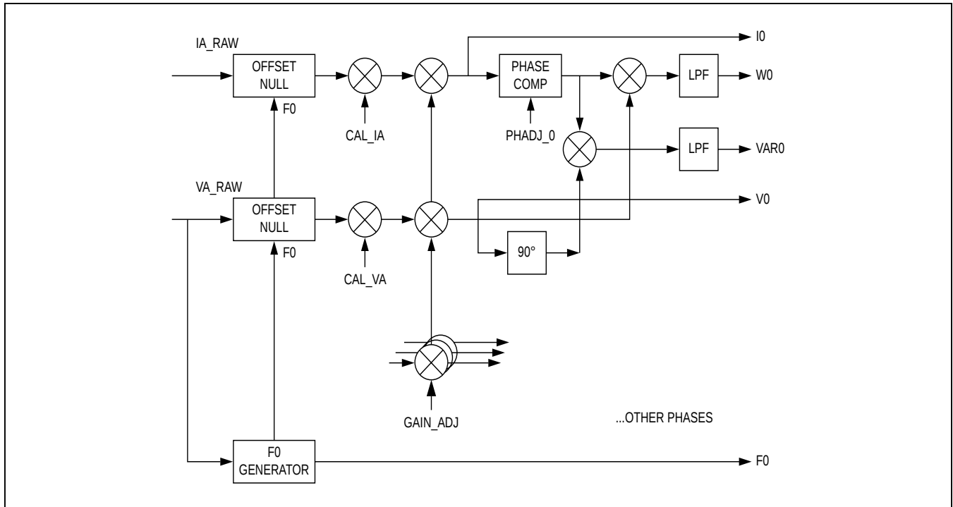
Figure 21. CE Data Flow – Offset, Gain, and Phase Compensation
