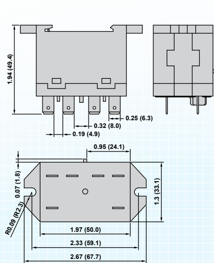
C3 – PANEL/DIN MOUNT (QC/SOLDER TERMINAL)
