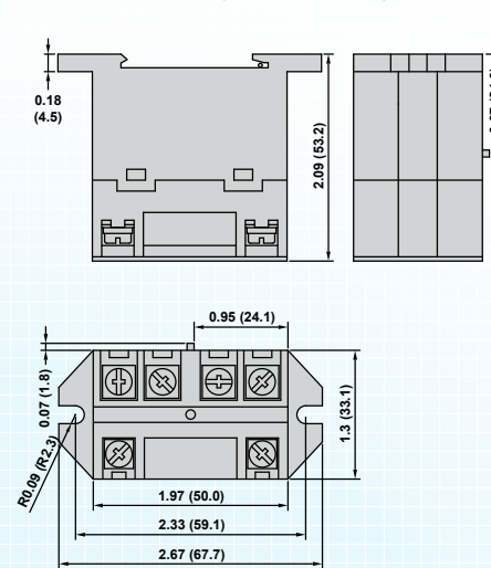
C3 – PANEL/DIN MOUNT (SCREW TERMINAL)
