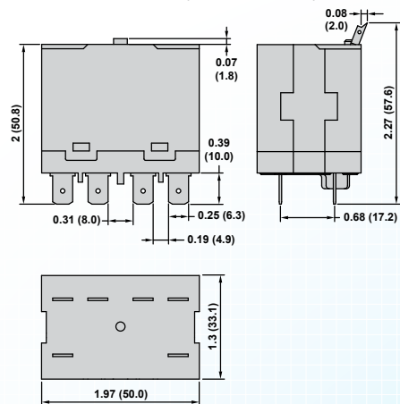
PLUG-IN SOCKET MOUNT (BLADE TERMINAL)
