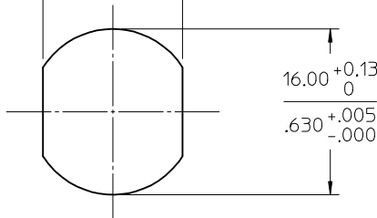
RECOMMENDED MOUNTING HOLE PATTERN
