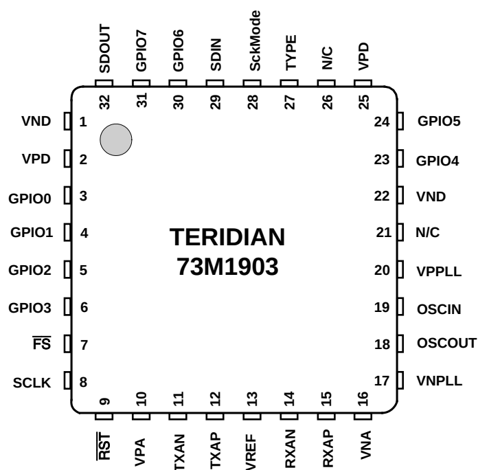
Figure 12: 32-Pin QFN Pinout
