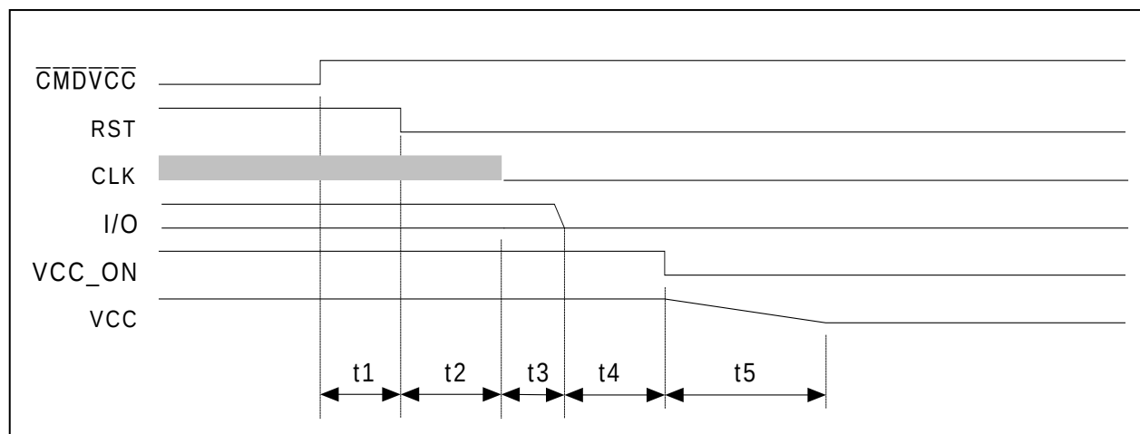
Figure 6: Deactivation Sequence
