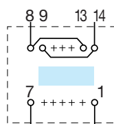
1 Secondary winding 8 9 13 14
