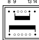
1 Secondary winding 8 9 13 14
