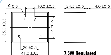
7.5W Regulated
