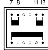
2 Secondary windings 7 8 11 12
