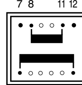
1 Secondary winding 7 8 11 12
