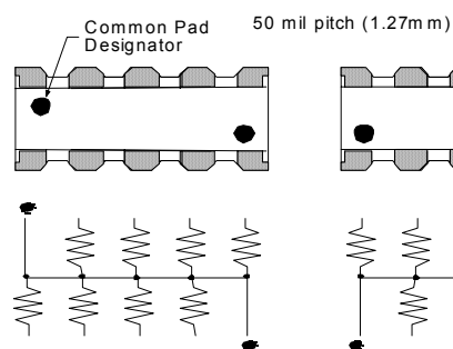
745X101 8 Resistors 10 Terminations
