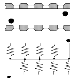
745X102 8 Resistors 10 Terminations
