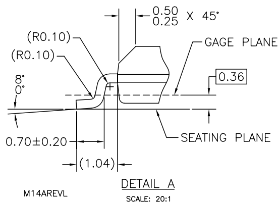
Figure 1. 14-Lead Small Outline Integrated Circuit (SOIC), JEDEC MS-012, 0.150" Narrow Package Number M14A
