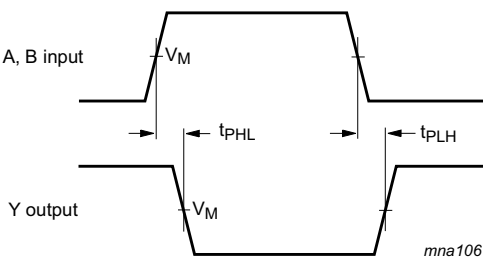
Fig 5. The inputs (A and B) to output (Y) propagation delays
