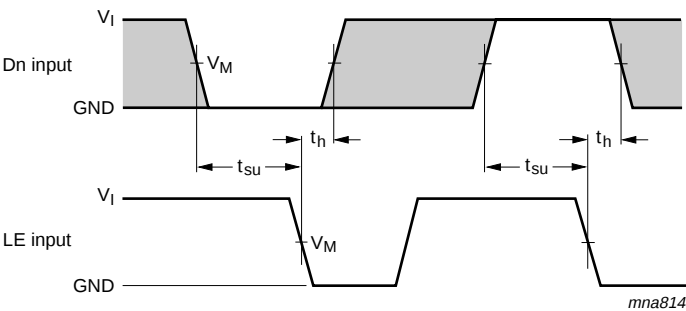
Measurement points are given in Table 8 . V OL and V OH are typical voltage output levels that occur with the output load. The shaded areas indicate when the input is permitted to change for predictable output performance.
