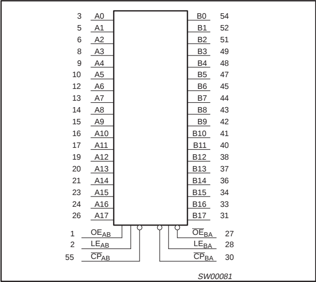
LOGIC SYMBOL
