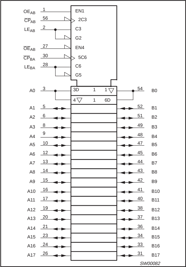
LOGIC SYMBOL (IEEE/IEC)
