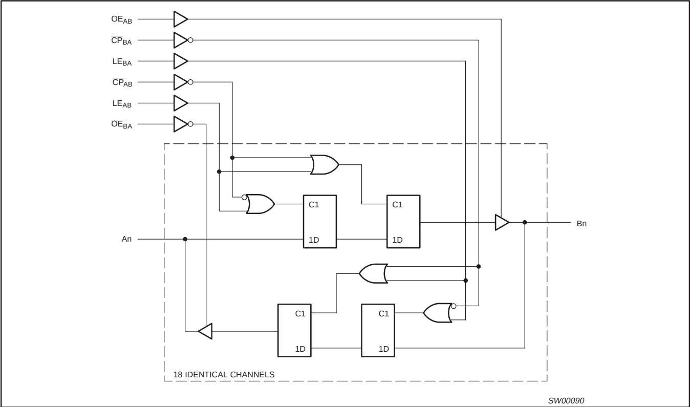
LOGIC DIAGRAM (one section)
