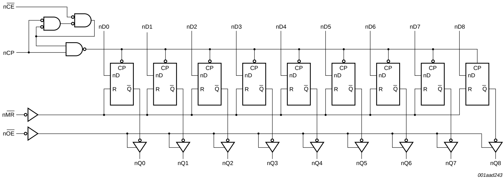
Fig 4. Logic diagram
