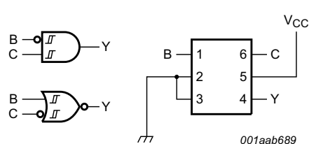
Fig 7. 2-input AND gate with inverted B input or 2-input NOR gate with inverted C input
