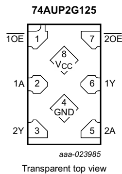
Fig 8. Pin configuration SOT1233
