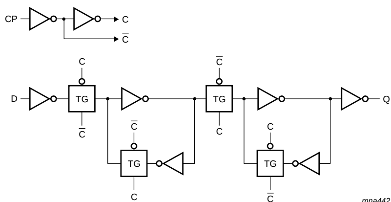
Fig 3. Logic diagram (one flip-flop)
