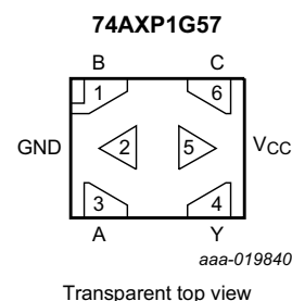
Fig 4. Pin configuration SOT1255 (X2SON6)
